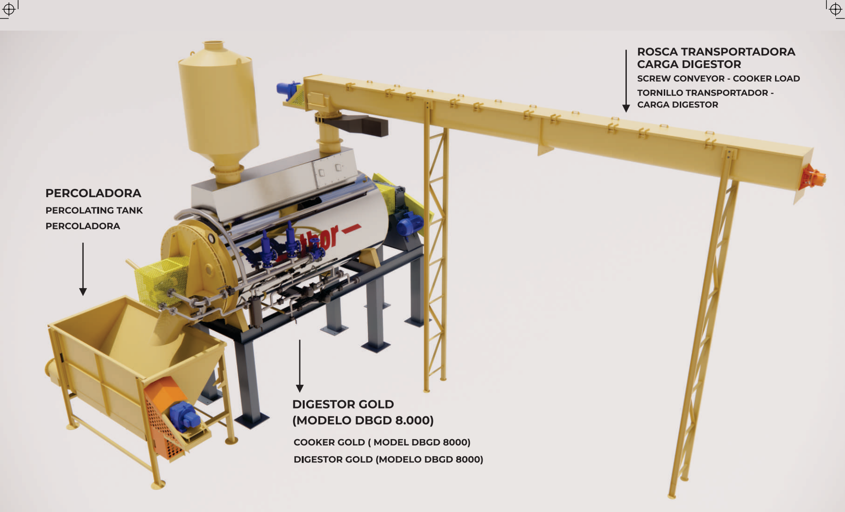
PROCESSADOR BATELADA GOLD (GOLD BATCH COOKER)
